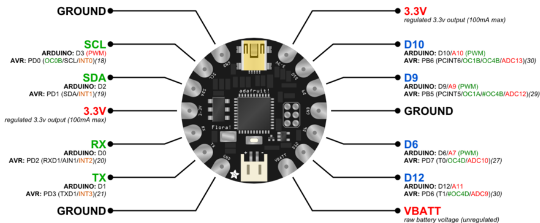
FLORA Wearable Electronics Platform adafruit.com/products/659
